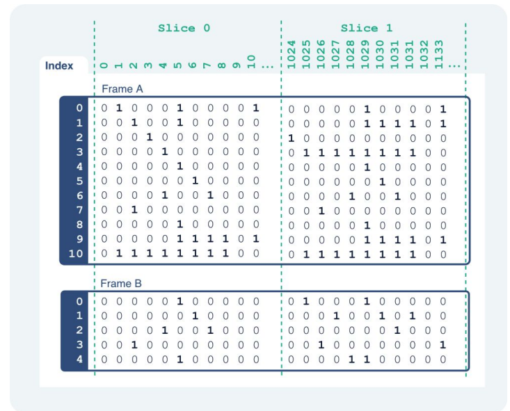
Figure 1: Illustration of the Pilosa data model, a binary index, showcasing groupings of columns called "frames."
